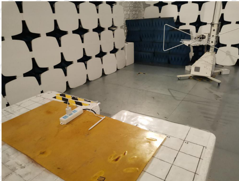
Photograph of test setup for Radiated disturbance
